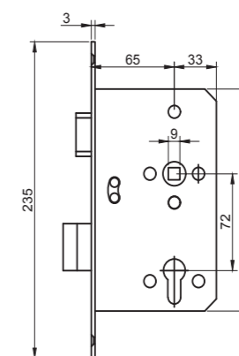
→ main lock
