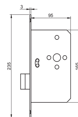
→ ancillary lock
