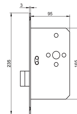
→ ancillary lock
