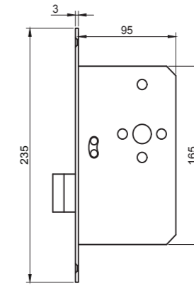
→ ancillary lock
