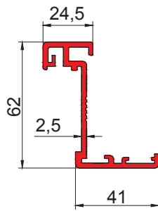
→ corner aluminium frame - general view
