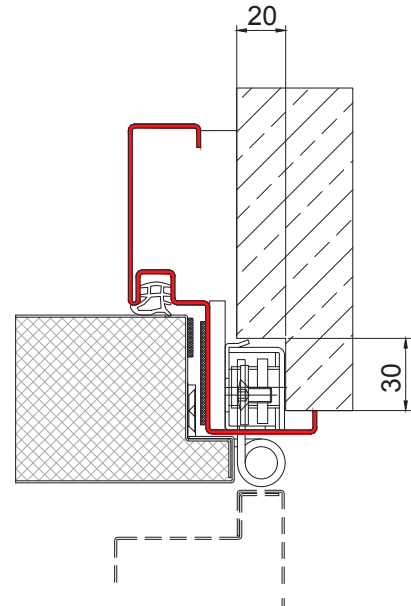
→ corner steel frame - hinge side view, 3D adjustable hinge - wall notched size 20 x 30 x 150 mm
