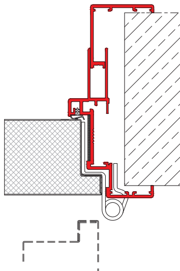
→ embracing frame for doors with hidden rebate - hinge side view, standard hinge
