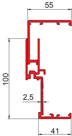
→ embracing aluminium frame - general view
