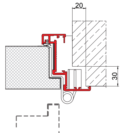
→ corner frame for doors with hidden rebate - hinge side view, 3D adjustable hinge - wall notched size 20 x 30 x 150 mm
