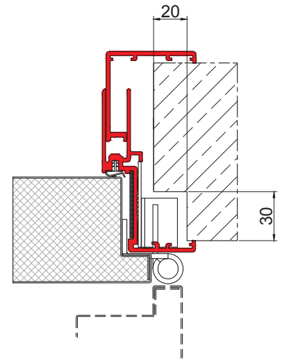
→ embracing frame - hinge side view, 3D adjustable hinge - wall notched size 20 x 30 x 150 mm
