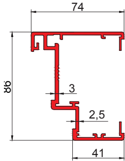
→ block aluminium frame for doors with hidden rebate – general view
