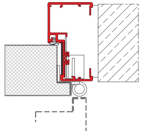
→ block frame with thermal break - hinge side view, 3D adjustable hinge
