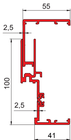
→ embracing aluminium frame with thermal break - general view
