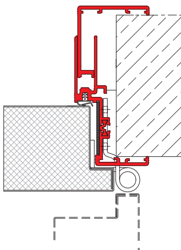
→ embracing frame with thermal break - hinge side view, standard hinge
