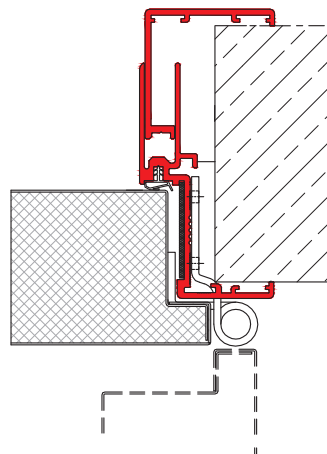
→ embracing frame - hinge side view, standard hinge
