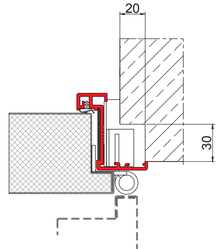
→ corner frame - hinge side view, 3D adjustable hinge - wall notched size 20 x 30 x 150 mm
