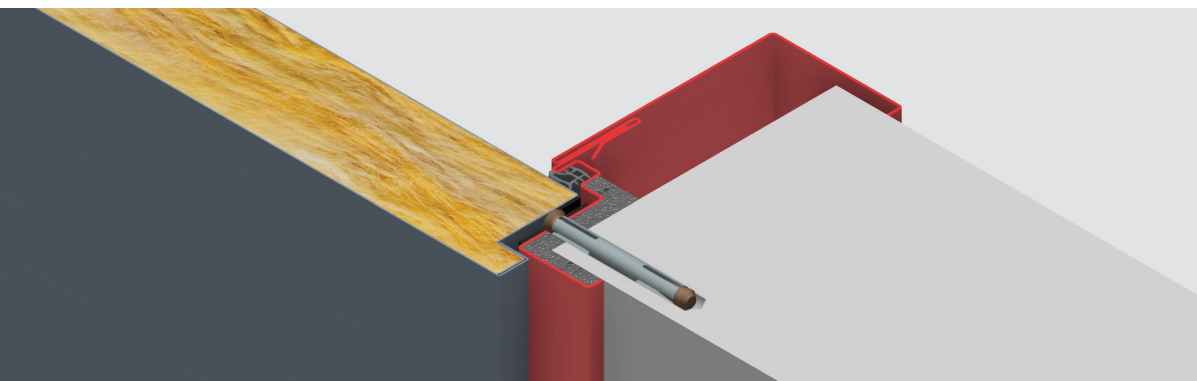
→ embracing steel frame - lock side view - wall notched size 20 x 30 x 170 mm
