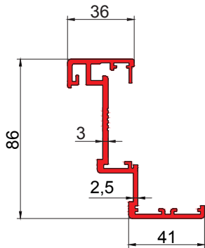
→ corner aluminium frame for doors with hidden rebate – general view
