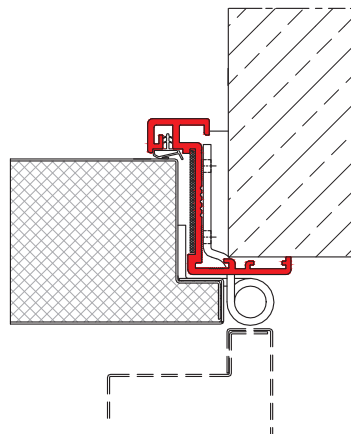
→ corner frame - hinge side view, standard hinge
