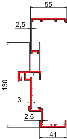
→ embracing aluminium frame for doors with hidden rebate – general view
