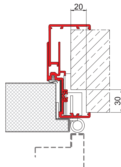
→ embracing frame with thermal break - hinge side view, 3D adjustable hinge - wall notched size 20 x 30 x 150 mm
