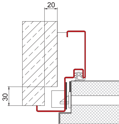
→ corner steel frame - general view
