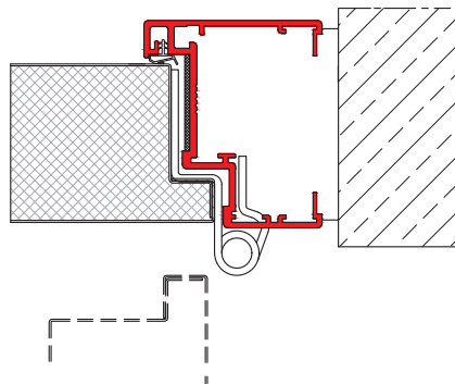
→ block frame for doors with hidden rebate – hinge side view, standard hinge
