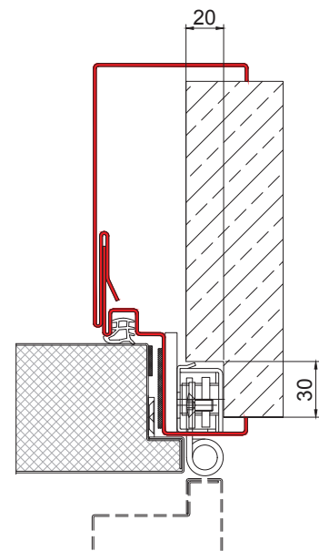
→ embracing steel frame - hinge side view, 3D adjustable hinge - wall notched size 20 x 30 x 150 mm
