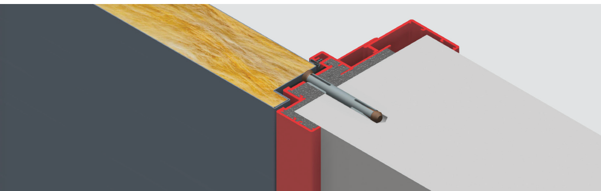
→ embracing frame for doors with hidden rebate - hinge side view, 3D adjustable hinge - wall notched size 20 x 30 x 150 mm
