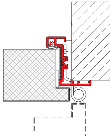
→ corner frame with thermal break - hinge side view, standard hinge
