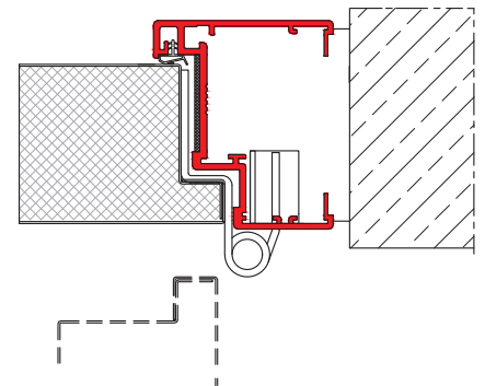
→ block frame for doors with hidden rebate – hinge side view, 3D adjustable hinge
