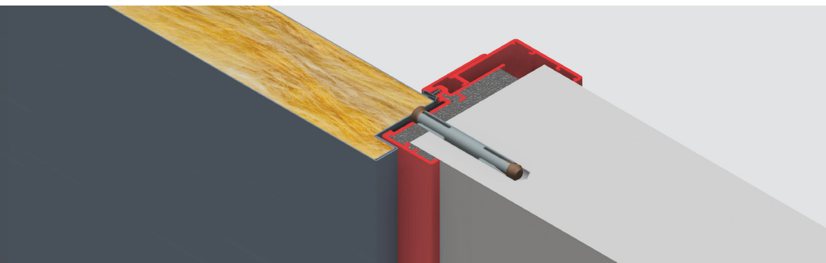
→ embracing frame - hinge side view, 3D adjustable hinge - wall notched size 20 x 30 x 150 mm
