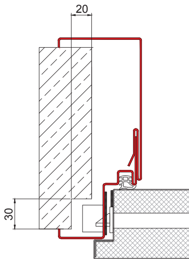
→ embracing steel frame - general view
