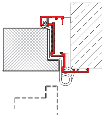
→ corner frame for doors with hidden rebate - hinge side view, standard hinge
