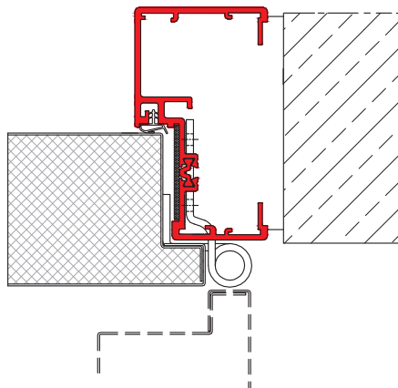
→ block frame with thermal break - hinge side view, standard hinge
