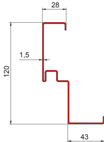
→ corner steel frame - general view
