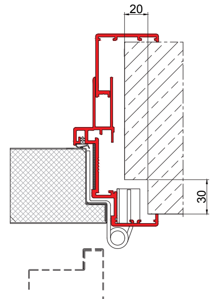
→ embracing frame for doors with hidden rebate - hinge side view, 3D adjustable hinge - wall notched size 20 x 30 x 150 mm
