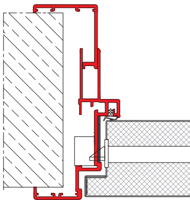
→ embracing aluminium frame for doors with hidden rebate – general view
